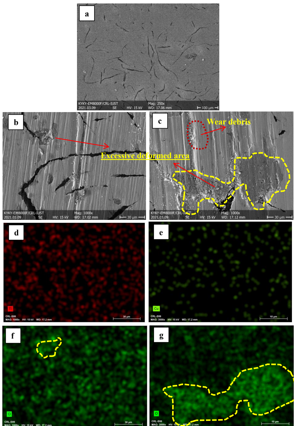
Fig. 13. SEM images of disc surface after wear test: (a) microstructure of The Grey cast iron, (b) wear track of the disc against the C0 pad, c) worn surface of the disc against the C7 pad, (d) and (f), X-ray elemental distribution of Ti and Oxygen on Brake disc against C0 brake pad, (e) and (g) X-ray elemental distribution of Ti and Oxygen on Brake disc against C0 brake pad.
